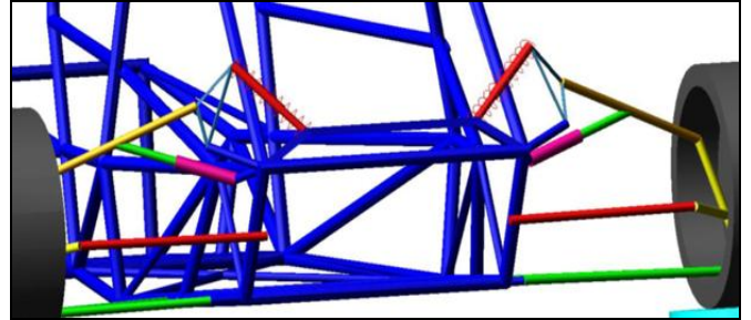
Fig. 4. The MBS model of the front axle suspension system (half-car model).
