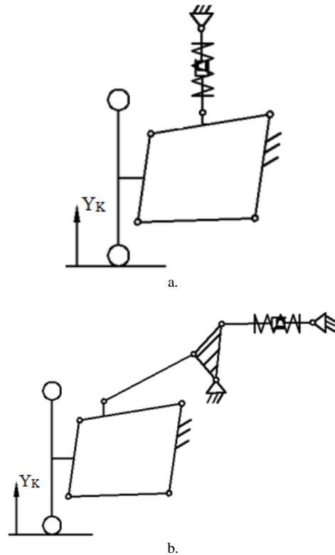
Fig. 1. The four-bar suspension mechanism: setups for passenger (a) and open-wheel (b) vehicles.
