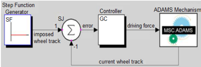
Fig. 5. Single-loop control scheme of the adaptive suspension mechanism.
