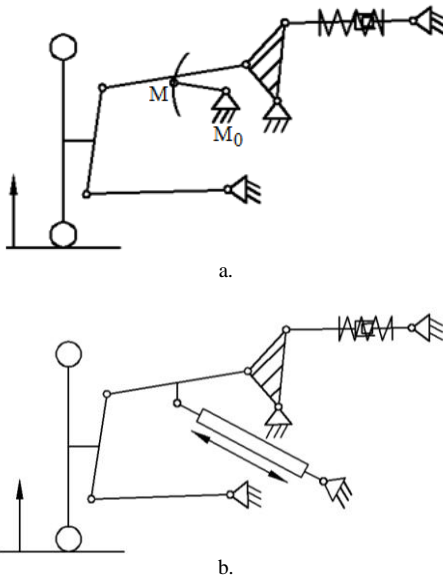
Fig. 3. The mono-mobile suspension systems derived from the five-bar mechanism: passive (a) and active (b).
