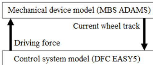
Fig. 6. Input & output plants in the mechatronic system.
