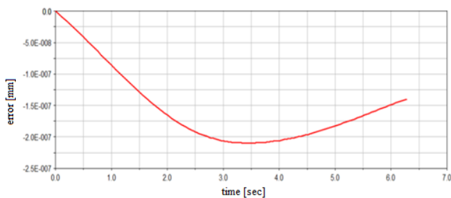
Fig. 8. The error obtained from the optimization of the PID controller.
