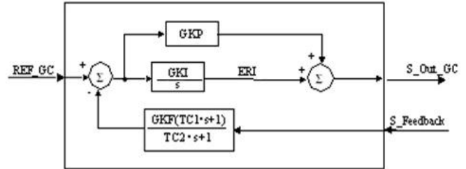
Fig. 7. Schematic model of the PID controller in EASY5 [21].
